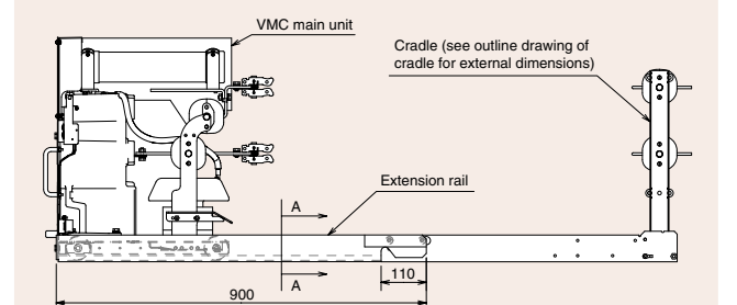
Figure 8.6 Extension rail
