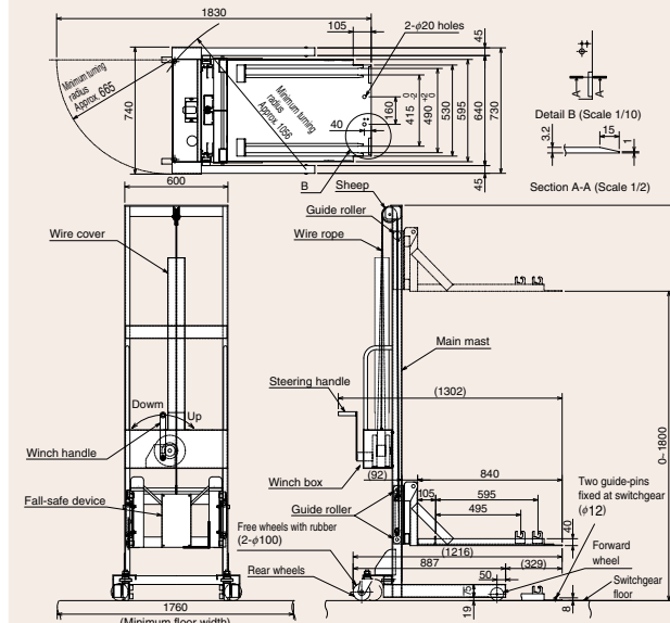
Figure 8.5 Lifter
